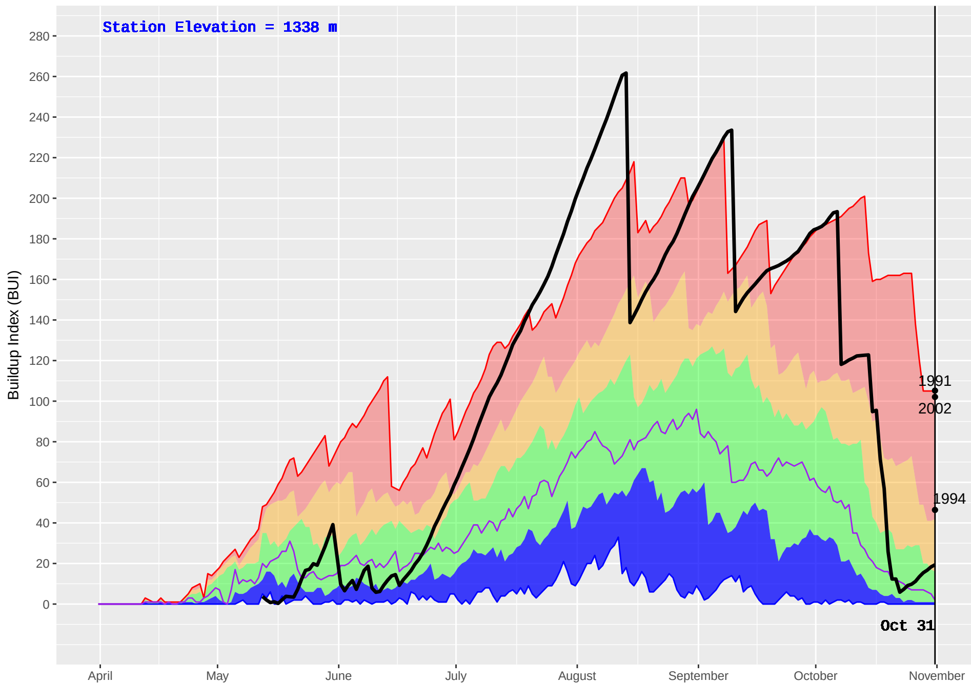
EIGHT MILE (391) : Historical (1980–2016) and Current (2017) Noon Buildup Index (BUI)
